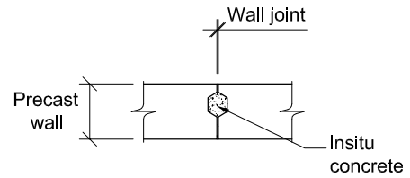
Plan of shear key at wall connection 1:50
