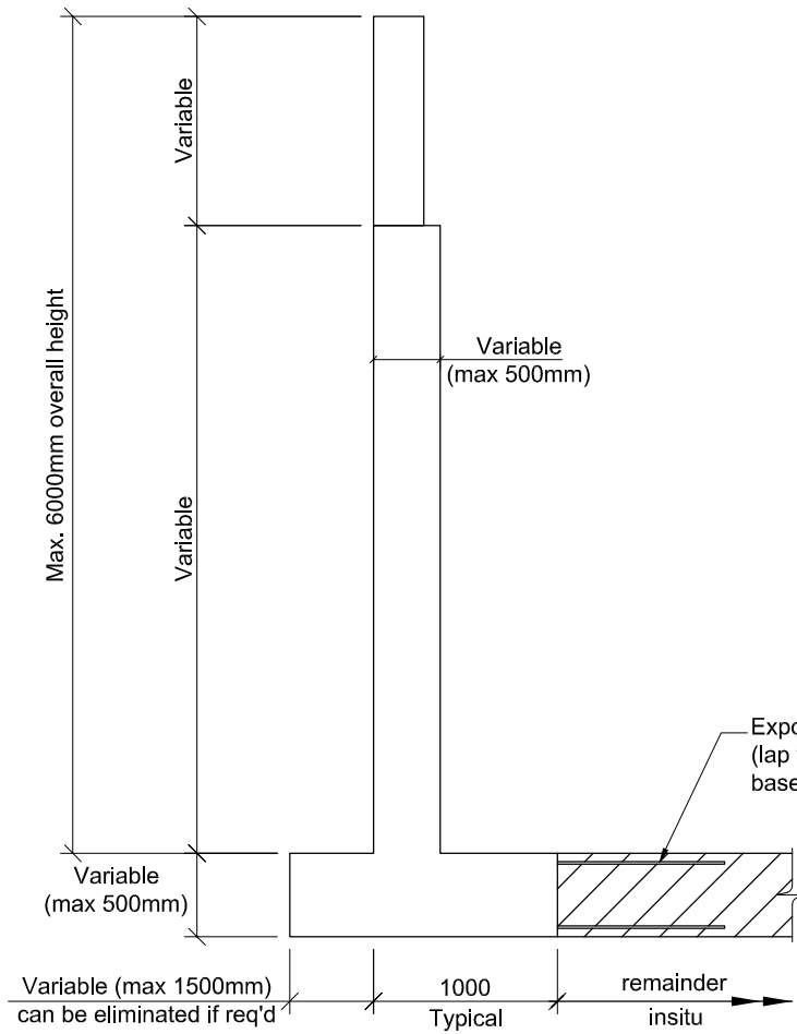
Section through wall 1:50
