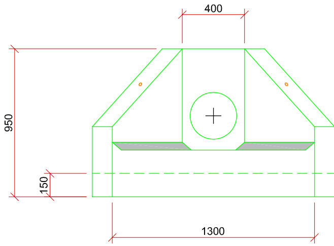
FRONT ELEVATION 1:25
